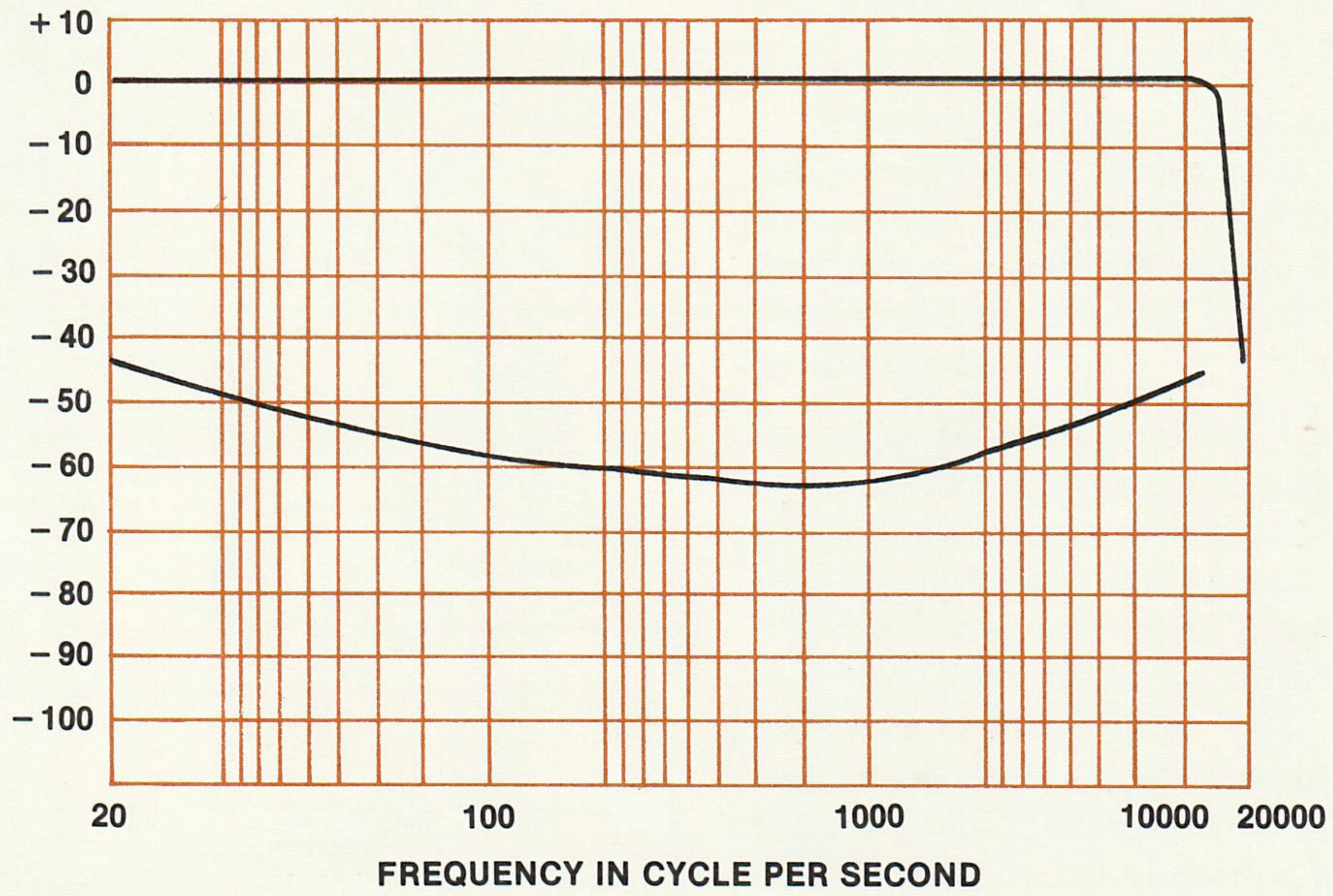
MR 500 FM FREQUENCY RESPONSE AND SEPARATION
