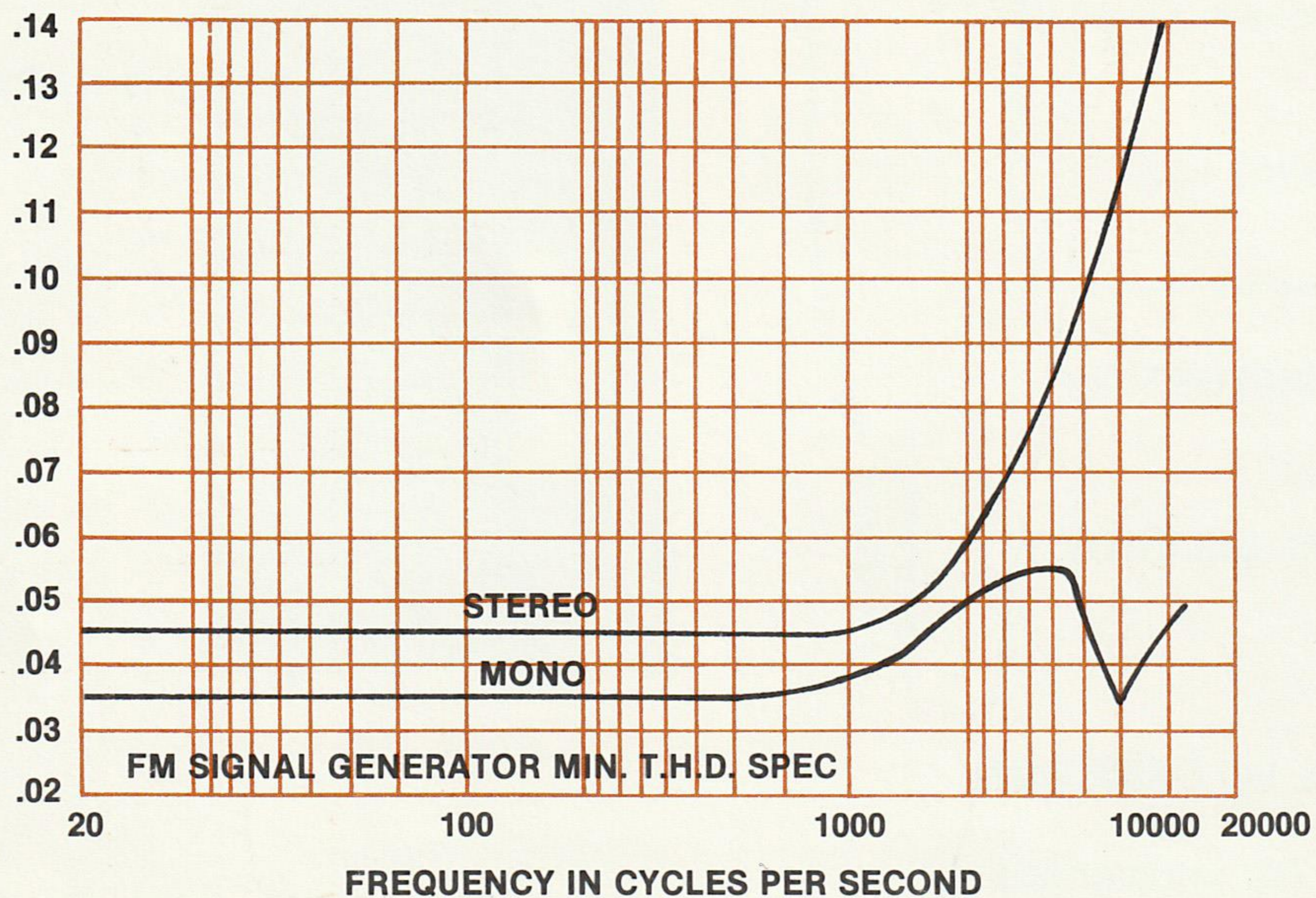
MR 500 T.H.D. @ 100% MODULATION 98 MHz
