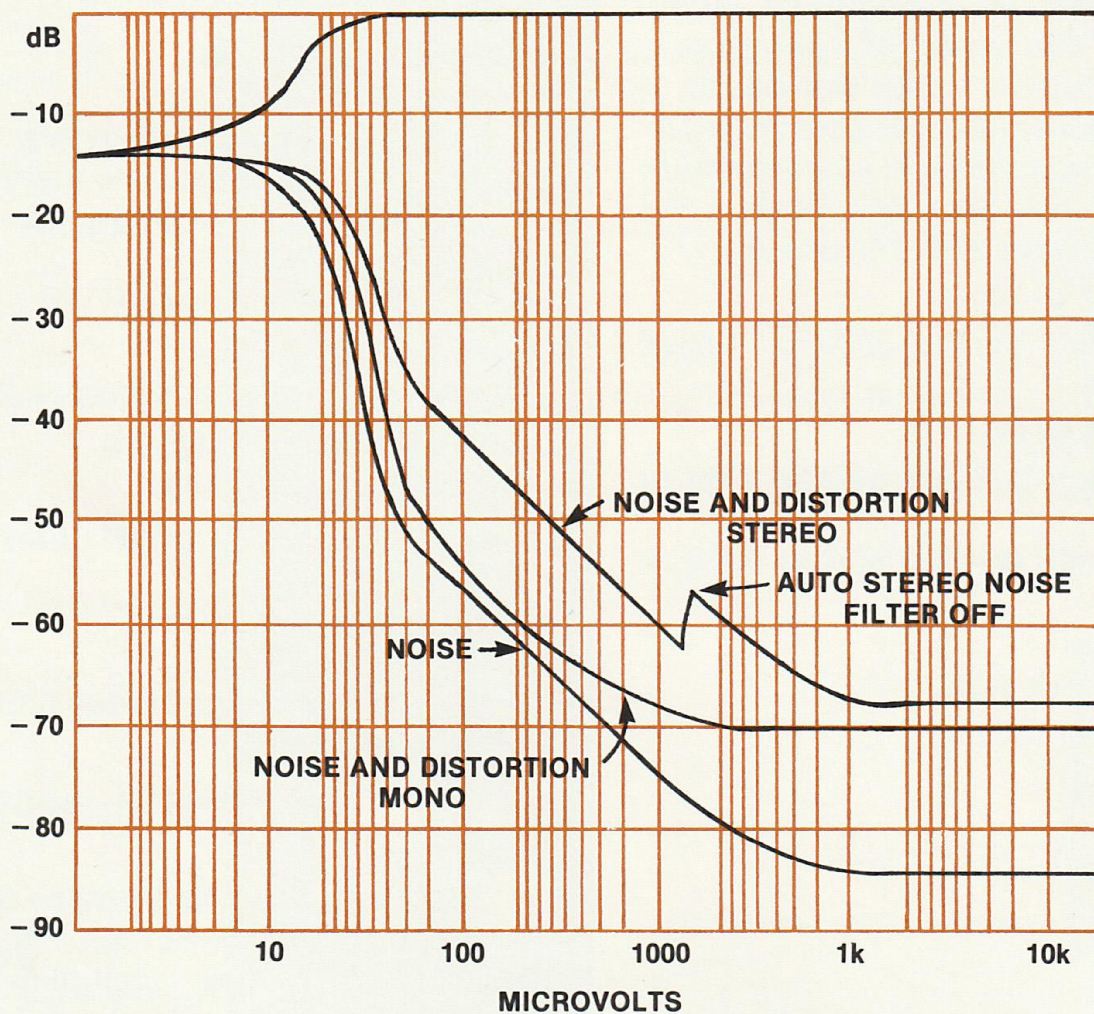
MR 500 FM SIGNAL PERFORMANCE 98 MHz, 1 kHz MOD 100%
