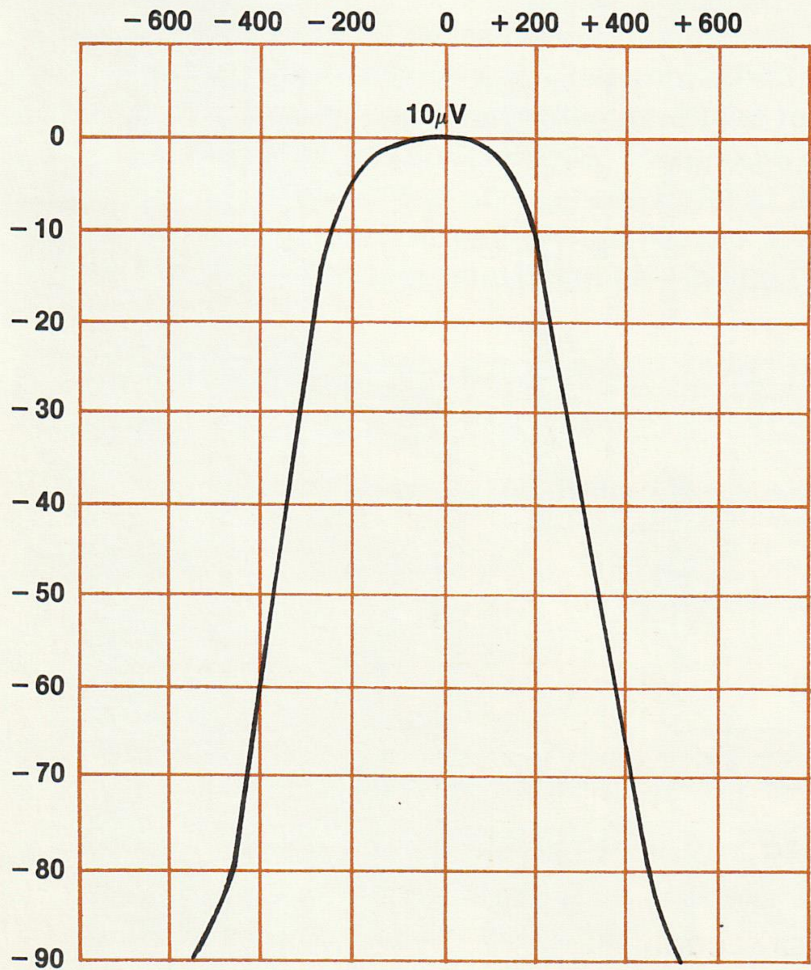
MR 500 SELECTIVITY DEV IN kHz
